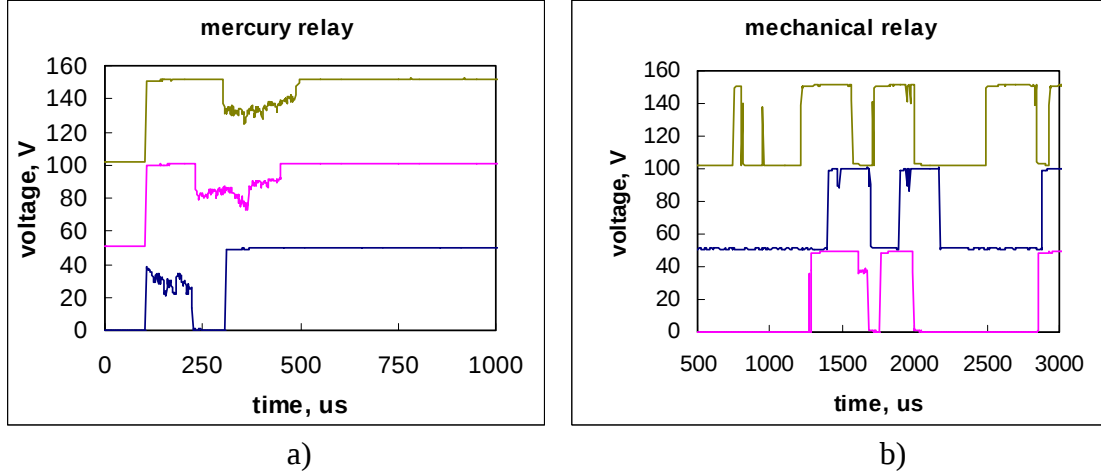
Figure 13. Voltage transients across a 100-Ohm resistor used as a replacement of capacitors in circuits with a mercury (a) and mechanical (b) relay. The curves are offset for better view of the transients.
