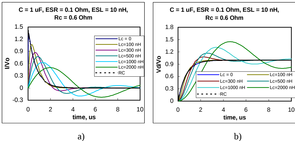
Figure 7. Simulation of current (a) and voltage across the dielectric (b) transients during surge testing for a 1 \mu\text{F} capacitor at different values of circuit inductance L_c . The resistance of the circuit, R_c = 0.6 \text{ Ohm} , was chosen in the middle of the range allowed per MIL-PRF-55365.
