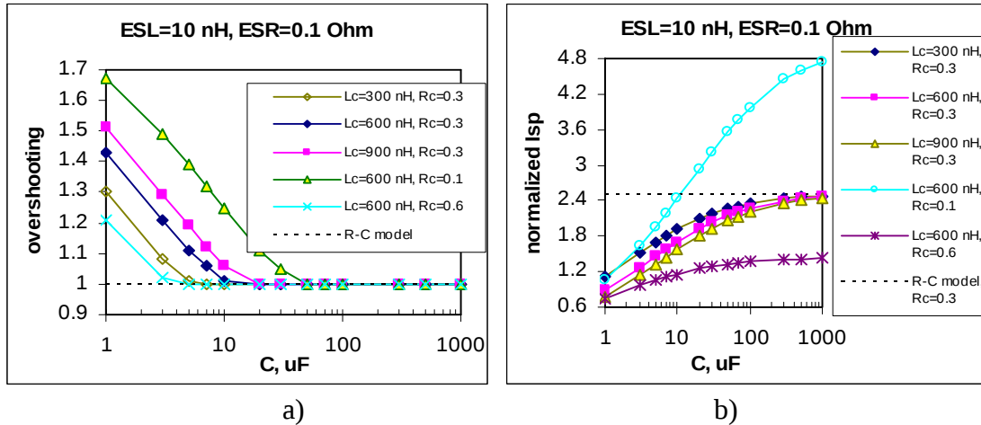
Figure 10. Effect of capacitance on overshooting (a) and current spike amplitude (b) according to R-C-L model. Dashed lines are results of calculations per R-C model.
