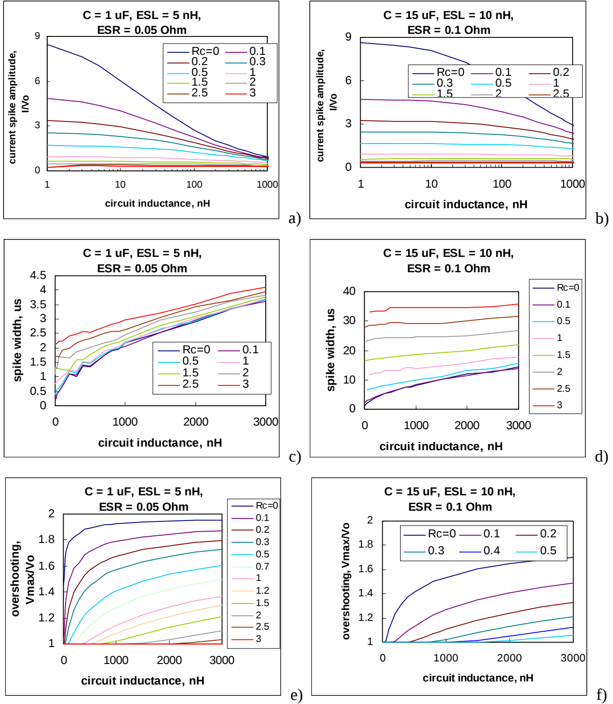
Figure 8. Effect of inductance and resistance of the circuit on the amplitude of current spike (a, b), spike duration (c, d), and overshooting (e, f) for a 1 \mu F (a, c, e) and 15 \mu F (b, d, f) capacitors. The legend shows values of R_c in Ohms.
