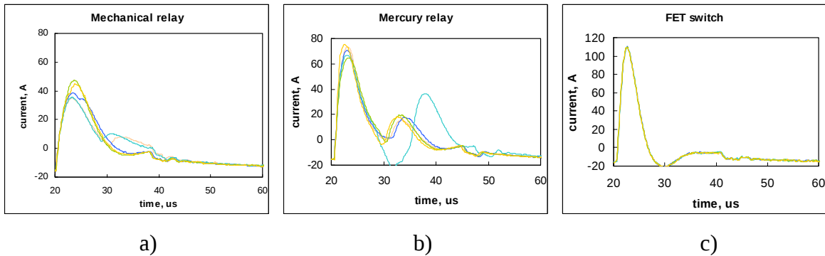
Figure 12. Reproducibility of current spikes in three set-ups with different types of switches: mechanical relay (a), mercury relay (b) and power FETs (c). The same 15 \mu\text{F}/50 \text{ V} tantalum capacitor was tested five times. No limiting resistors were used.
